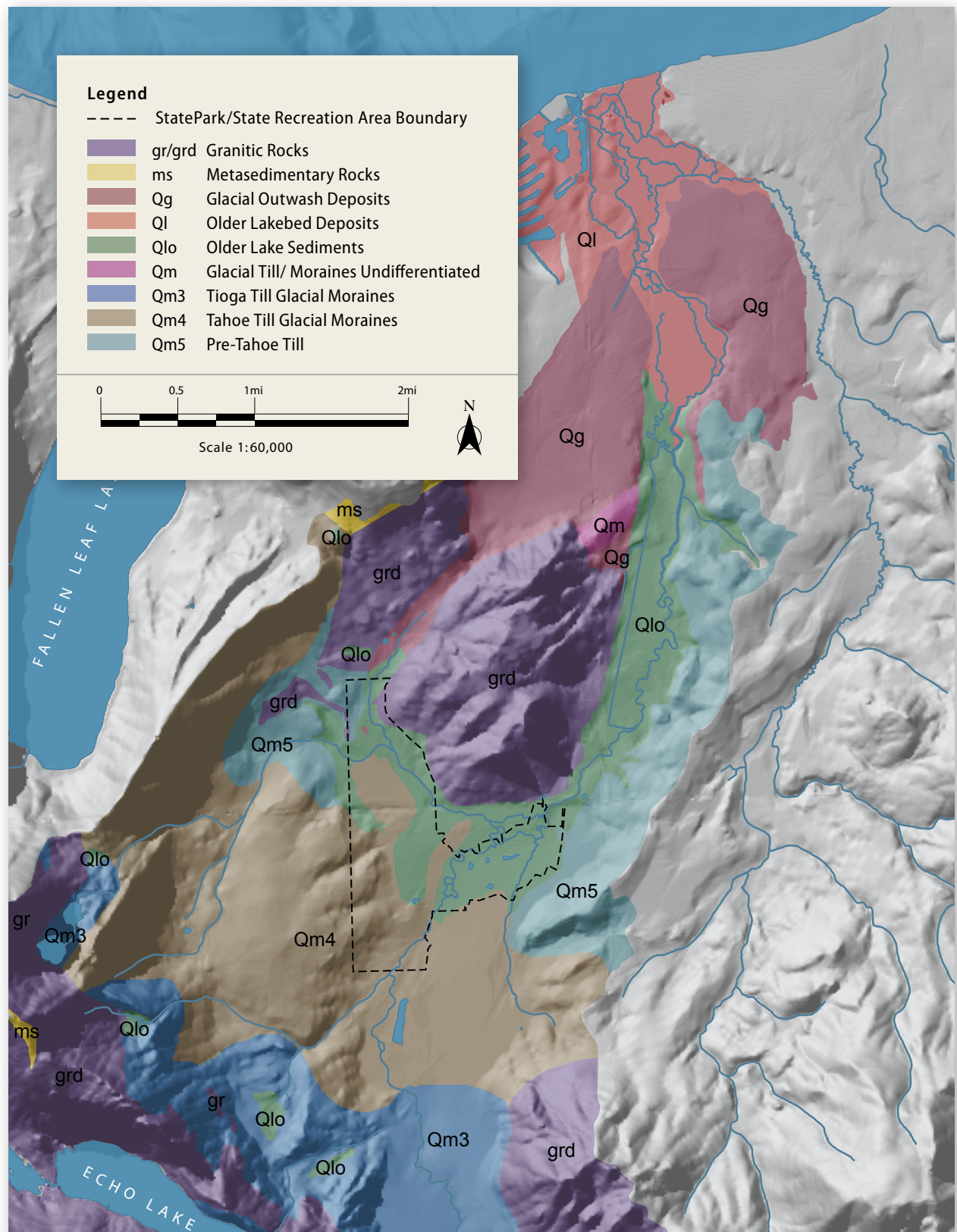
Figure 2: Upper Truckee River Geology
