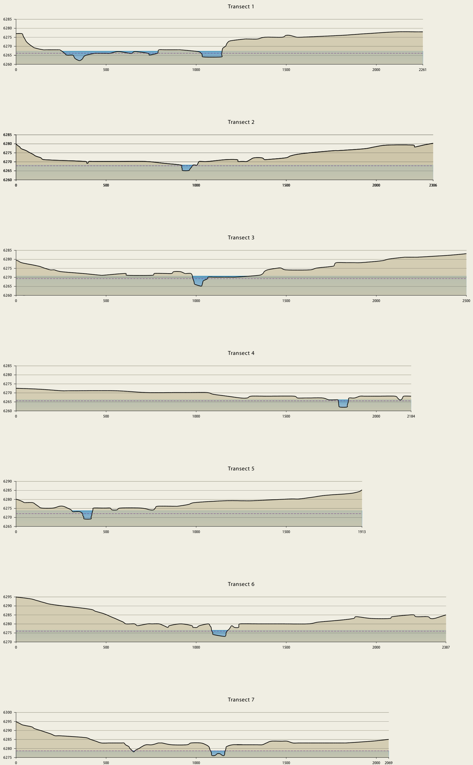
Figure 21: Upper Truckee Transects, 550cfs Estimated changes in water surface elevation, plotted on valley sections (Figure 20).
