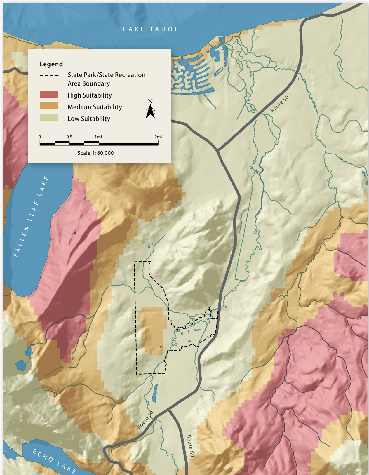
Figure 28: Current Pine Marten Habitat Suitability
