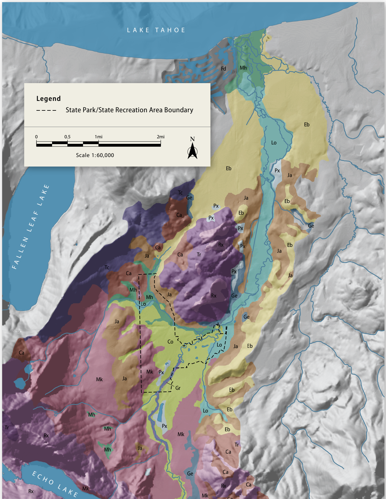
Figure 3a: Upper Truckee River Soils Legend and soil descriptions found on Figure 3b.
